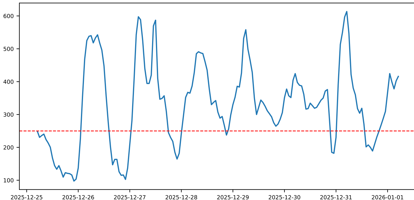
Ward PM2.5 (hourly mean, station data)
