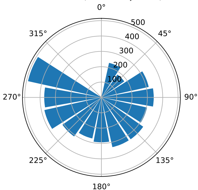
Pollution rose (mean PM2.5 by wind dir)
